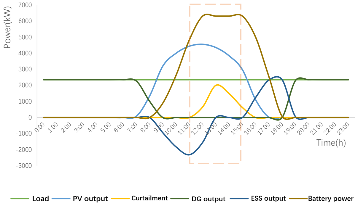
Fig. 4 Day-ESS is full charged
