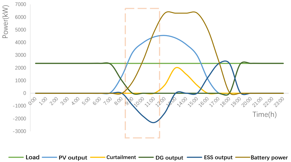
Fig. 3 Day-ESS is charged from PV
